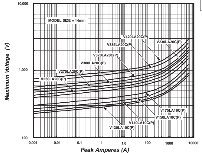
Figure 4. Maximum Clamping Voltage for 14mm Parts (V130LA10C(P) -V420LA20C(P))
