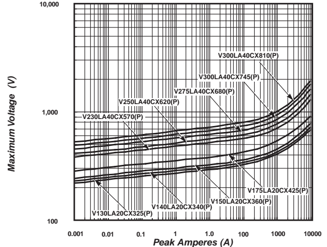
Figure 6. Maximum Clamping Voltage for Low Clamping Voltage Parts (V130LA20CX325(P) -V300LA40CX245(P))
